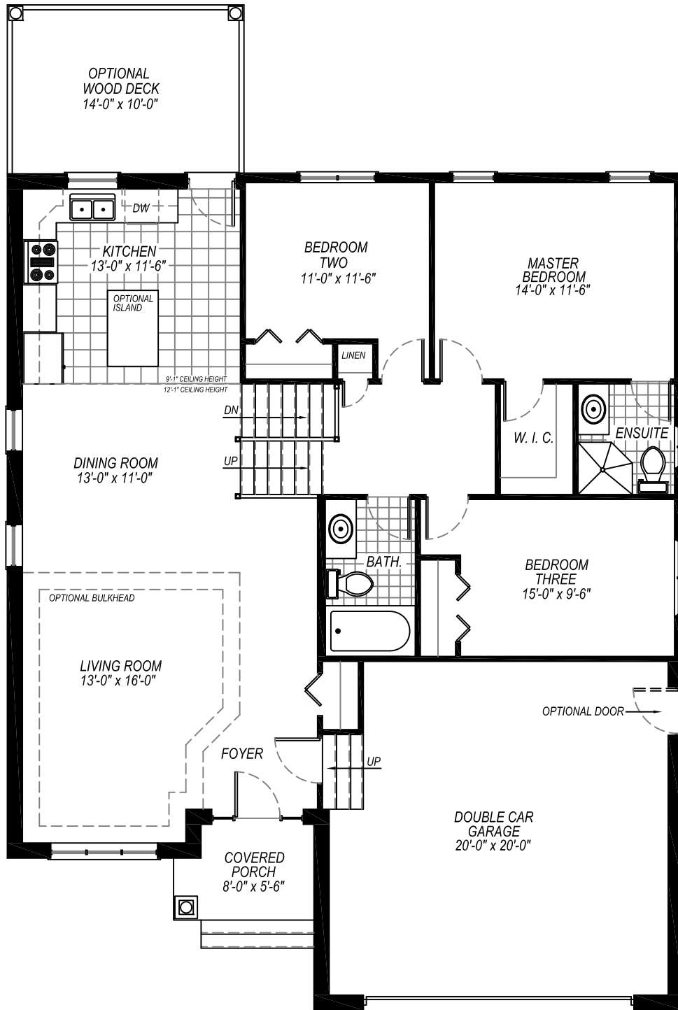
Main Floor Plan Approximately 2,035 sq.ft. Approximately 40'-0" x 49'-6" Optional 9'-0" ceiling
