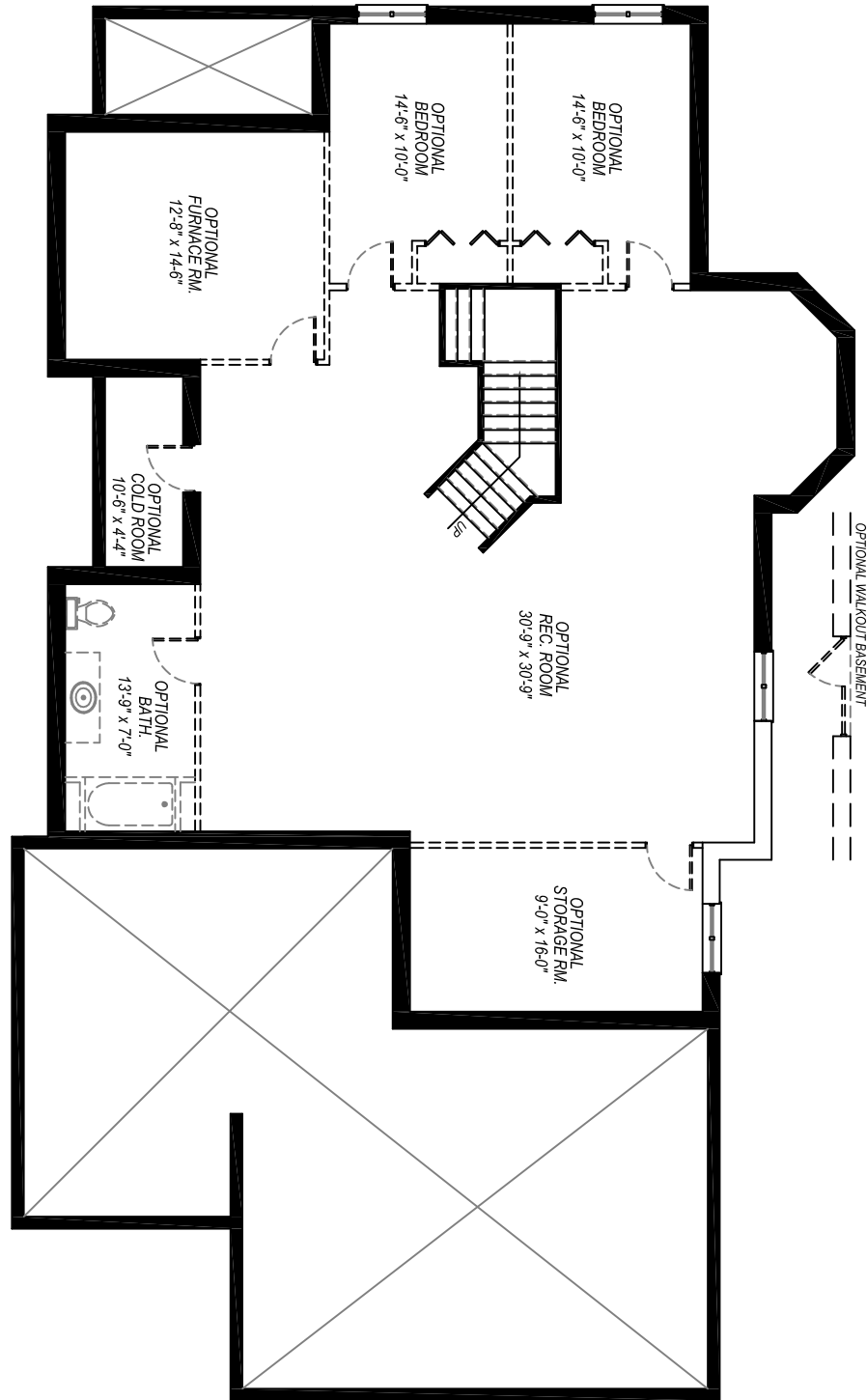
Lower Level Plan Approximately 3,890 sq.ft. Approximately 78'-0" x 47'-0" Optional 9'-0" ceiling
