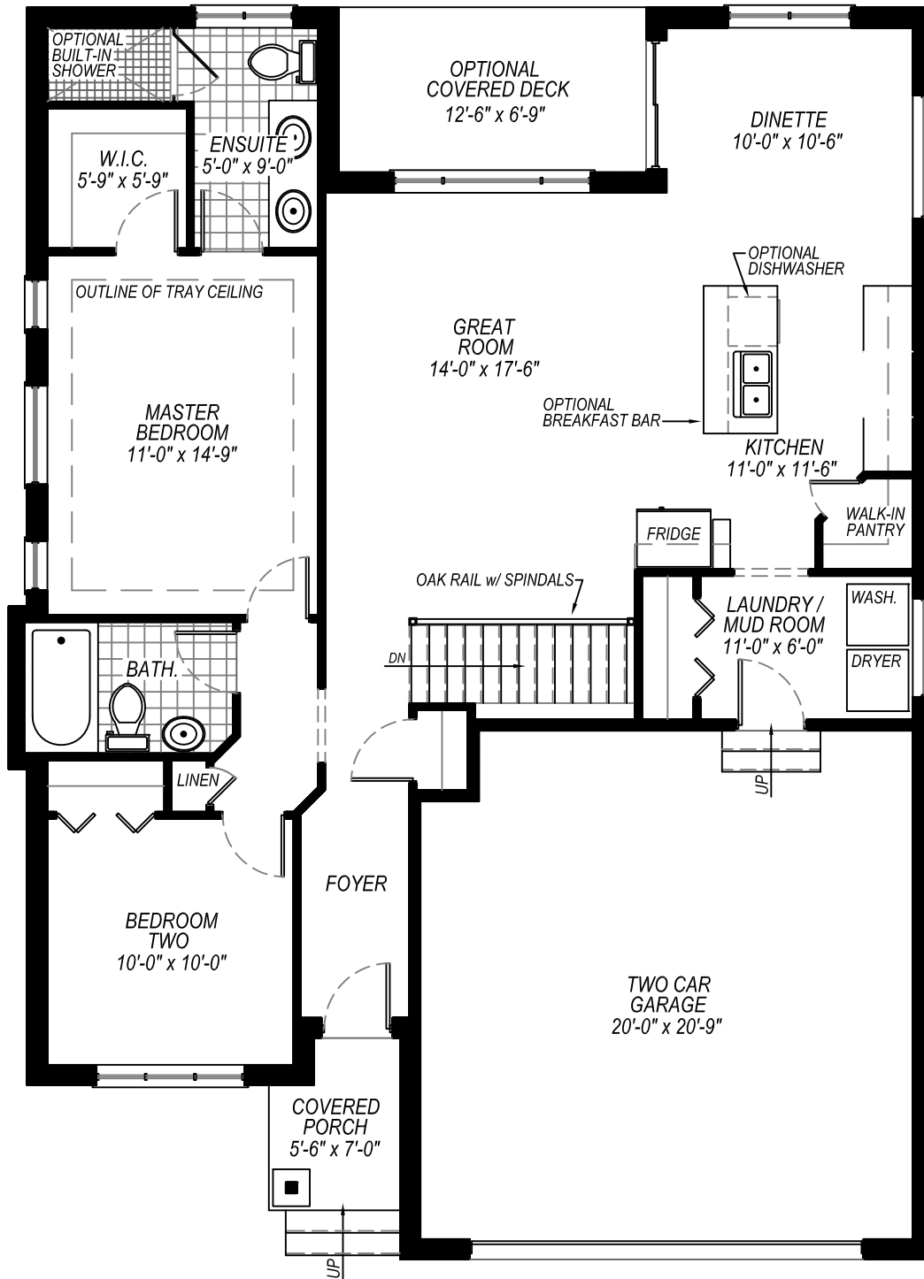
Main Floor Plan Approximately 1,235 sq.ft. Approximately 37'-0" x 51'-0" Optional 9'-0" ceiling
